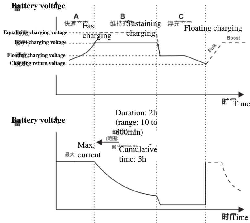
Fig. 1-5 Battery charging stages diagram
