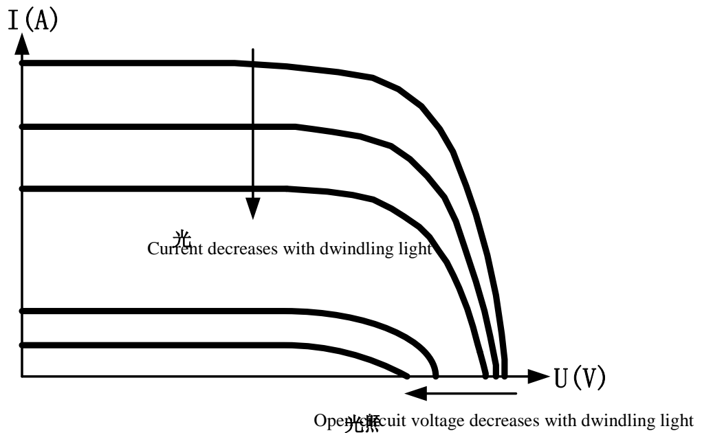
Fig. 1-3 Relation between solar panel output characteristics and illumination
